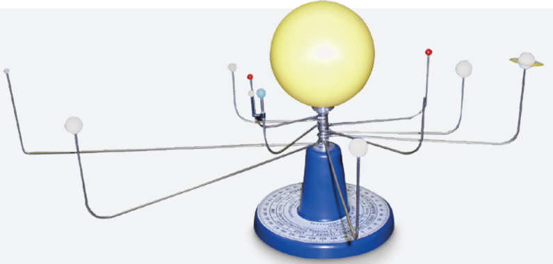
Trippensee® Solar System Model Copernican heliocentric solar system illustrates the motions of the planets, their relative sizes, and their relative distances from one another. All stainless-steel wire arms. Includes 10 orbits (8 planets, moon, and asteroid belt), instruction book with diagrams, and activities. SB15350 — $129.95
