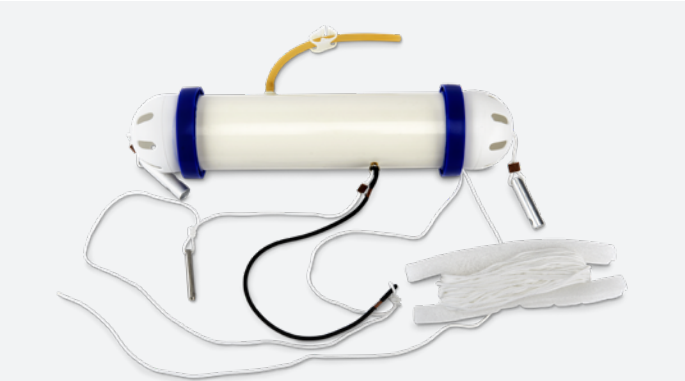
Water Sampler Sample water from any desired depth. Single-line trigger mechanism uses one line to both raise and lower the sampler and a trigger to seal the collection chamber; eliminating tangled lines. Flow-through design provides 1.5-liter volume of water from which temperature and dissolved oxygen content can be determined. 18½"L x 3½" dia. SB21418 – $81.95
