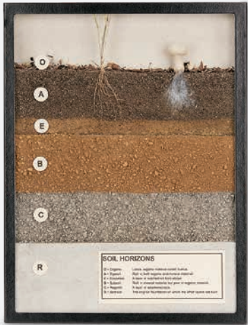
Soil Horizons Presents and defines each layer of soil (organic, topsoil, eluviation, subsoil, regolith, bedrock). Display is topped off with a stem of grass showing the roots, as well as a mushroom with mycelium extending into topsoil. 12" x 16". C34457 – $194.95
